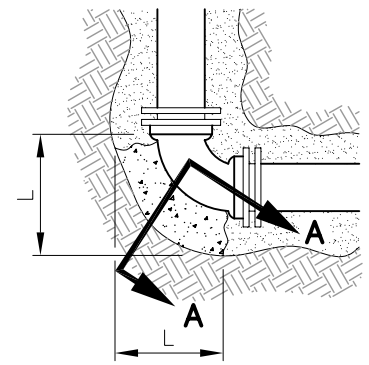
HORIZONTAL BEND
