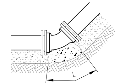
VERTICAL UNDER BEND
