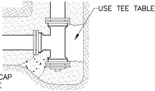
TEE W/ ONE PLUG END
